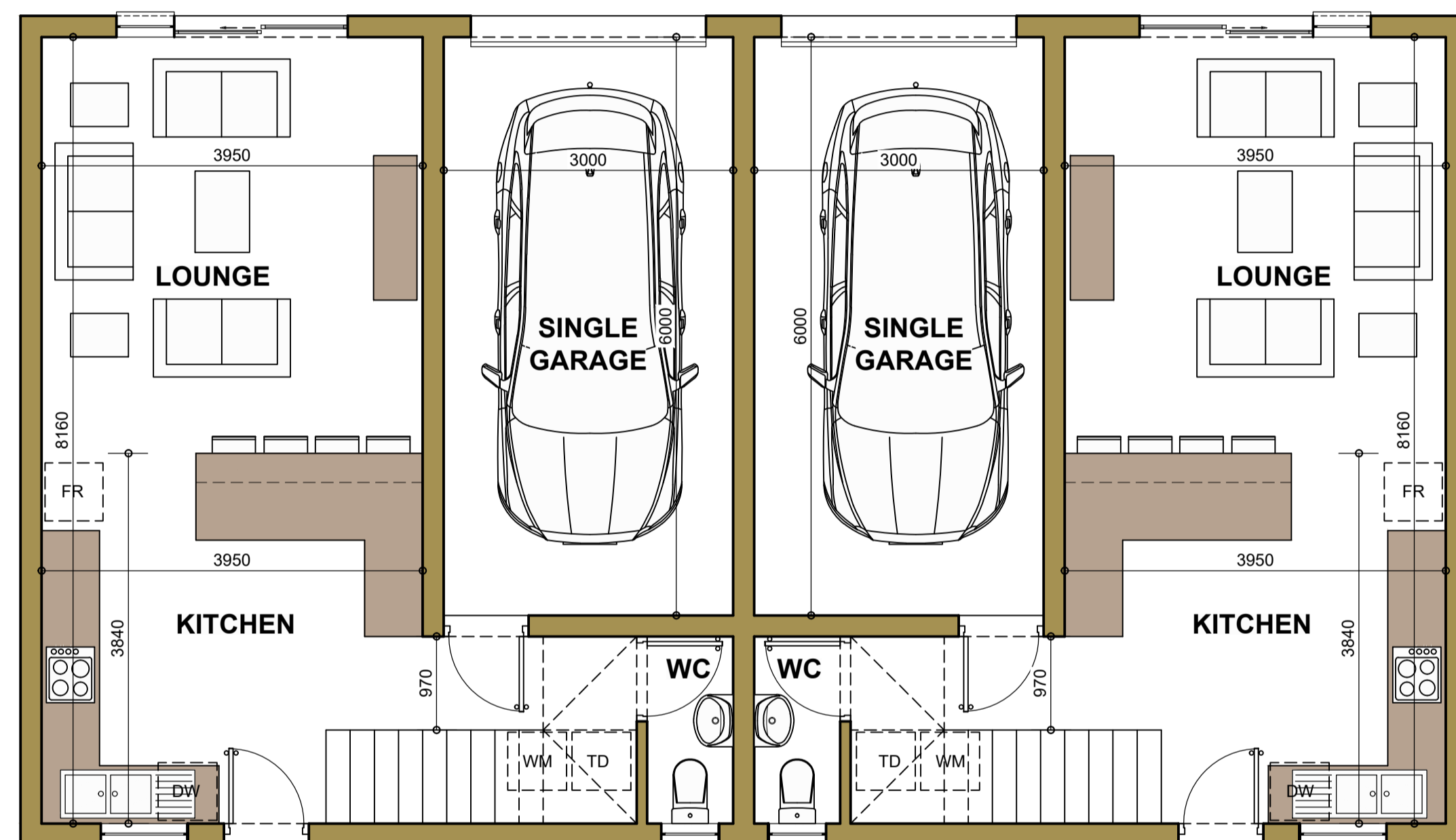
GROUND STOREY PLAN SCALE 1:50
