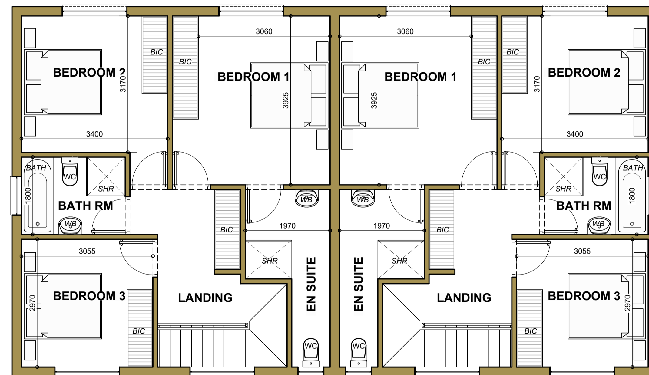
FIRST STOREY PLAN SCALE 1:50
